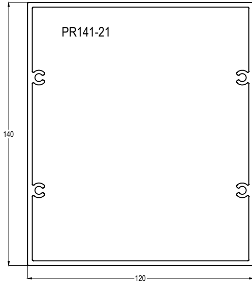
AB40T-ISI YALITIMLI CAM BALKON SİSTEMİ Glass Balcony System With Thermal Glass
